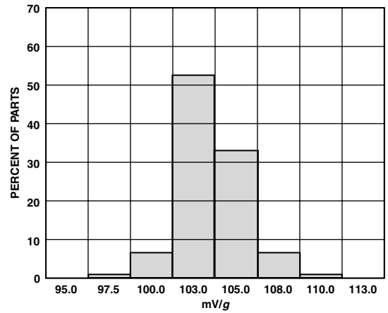
TPC 10. Y-Axis Sensitivity Distribution at Y_{FILTER} , V_{DD} = 5V
