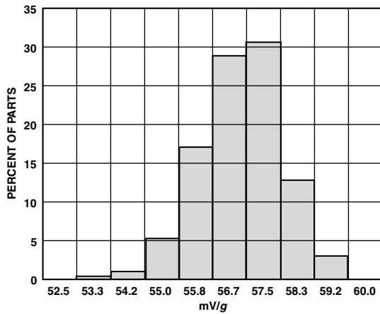
TPC 7. Y-Axis Sensitivity Distribution at Y_{FILTER} , V_{DD} = 3V
